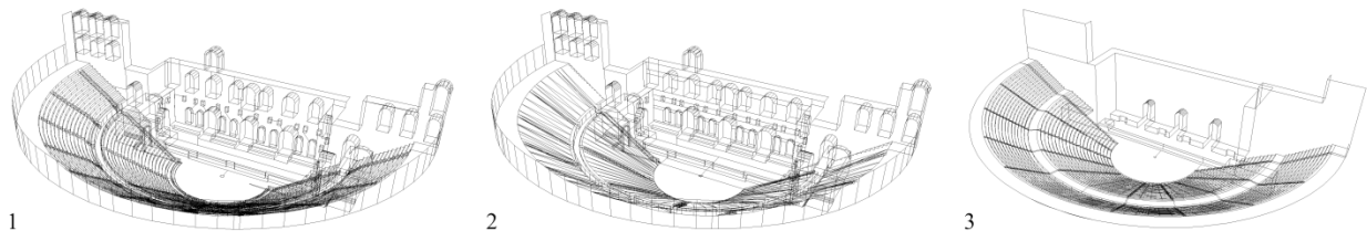
Figure 1. Wireframes visualizations of the Odeon of Herodes Atticus as obtained by Odeon (software). From left to right, the detailed model (1), the simplified model (2), and the model recreated from literature [6] (3).
